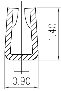
SECTION C-C
